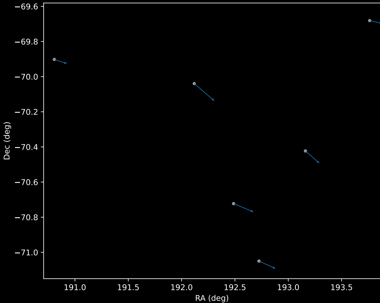
GALAH DR4 Cluster 0 Proper Motion Vectors (n=6)
