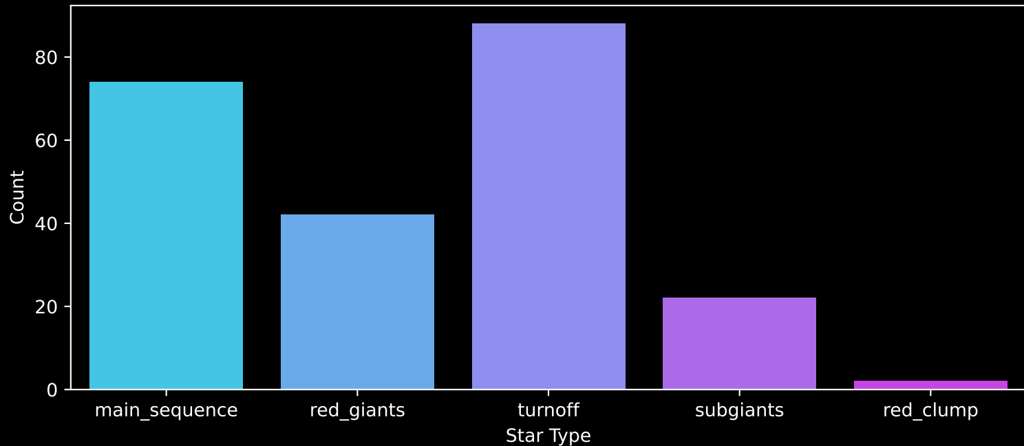
GALAH DR4 Field: [7133] Count plot of Star Type
