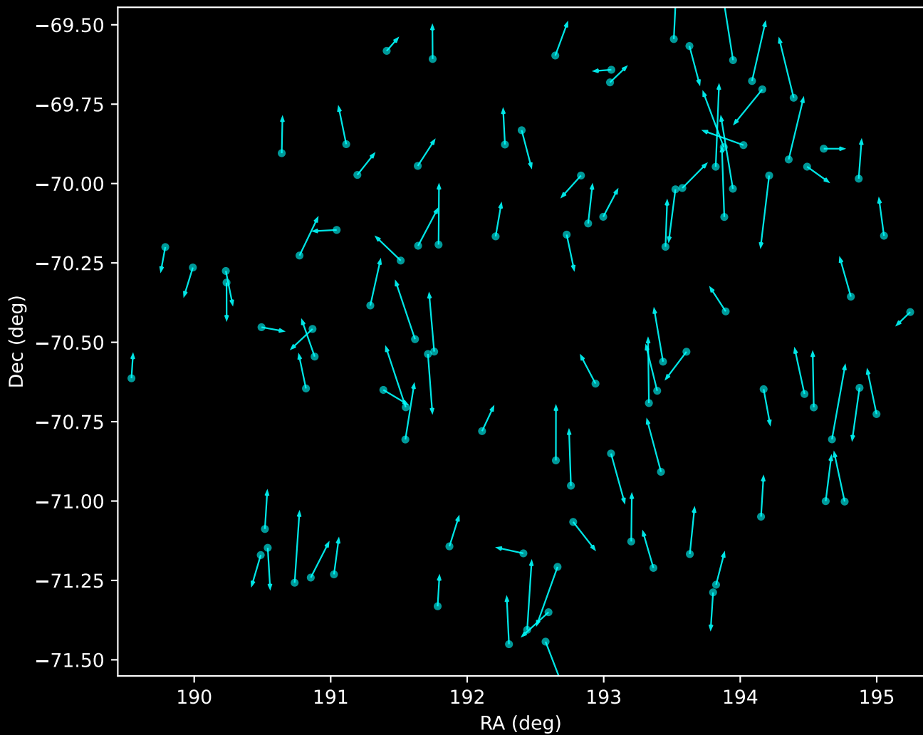
GALAH DR4 Noise Stream Proper Motion Vectors (n=99)
