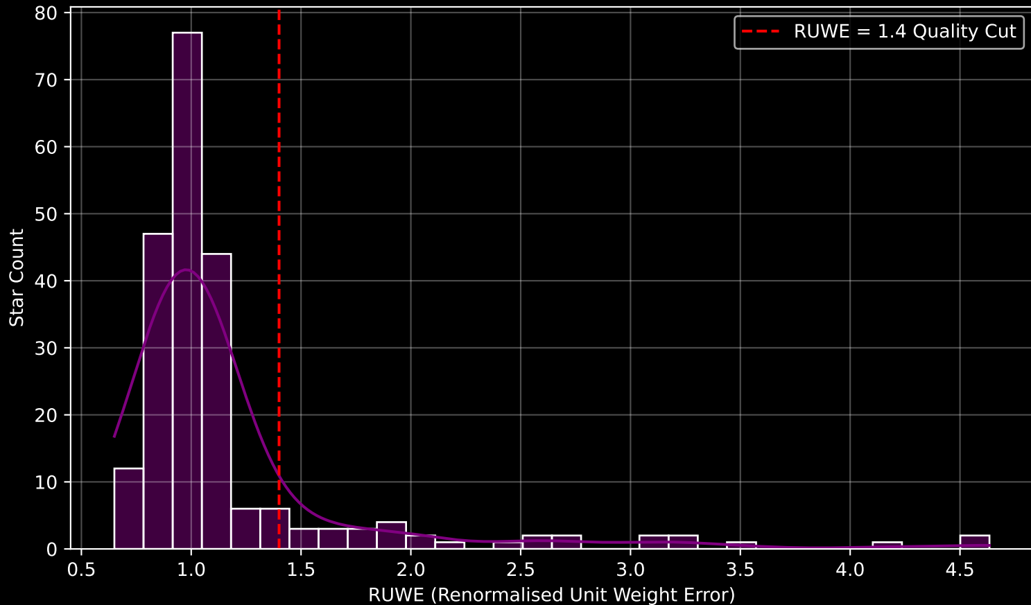
GALAH DR4 Field [7133] RUWE Distribution (n= 221)
