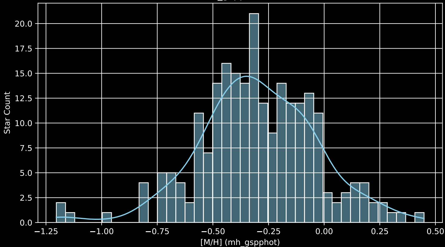
GALAH DR4 Field: [7133] [M/H] (mh_gspphot) (n= 228)
