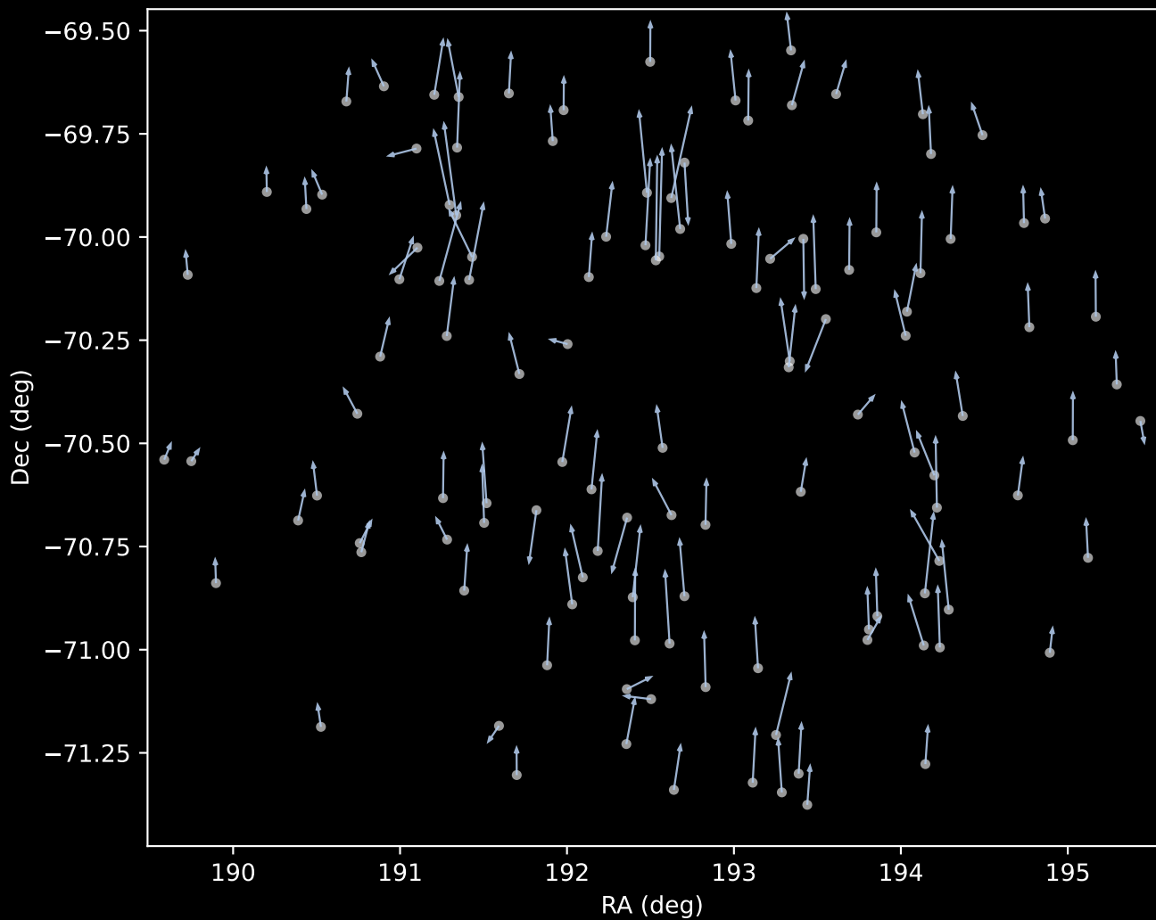
GALAH DR4 Cluster 1 Proper Motion Vectors (n=123)
