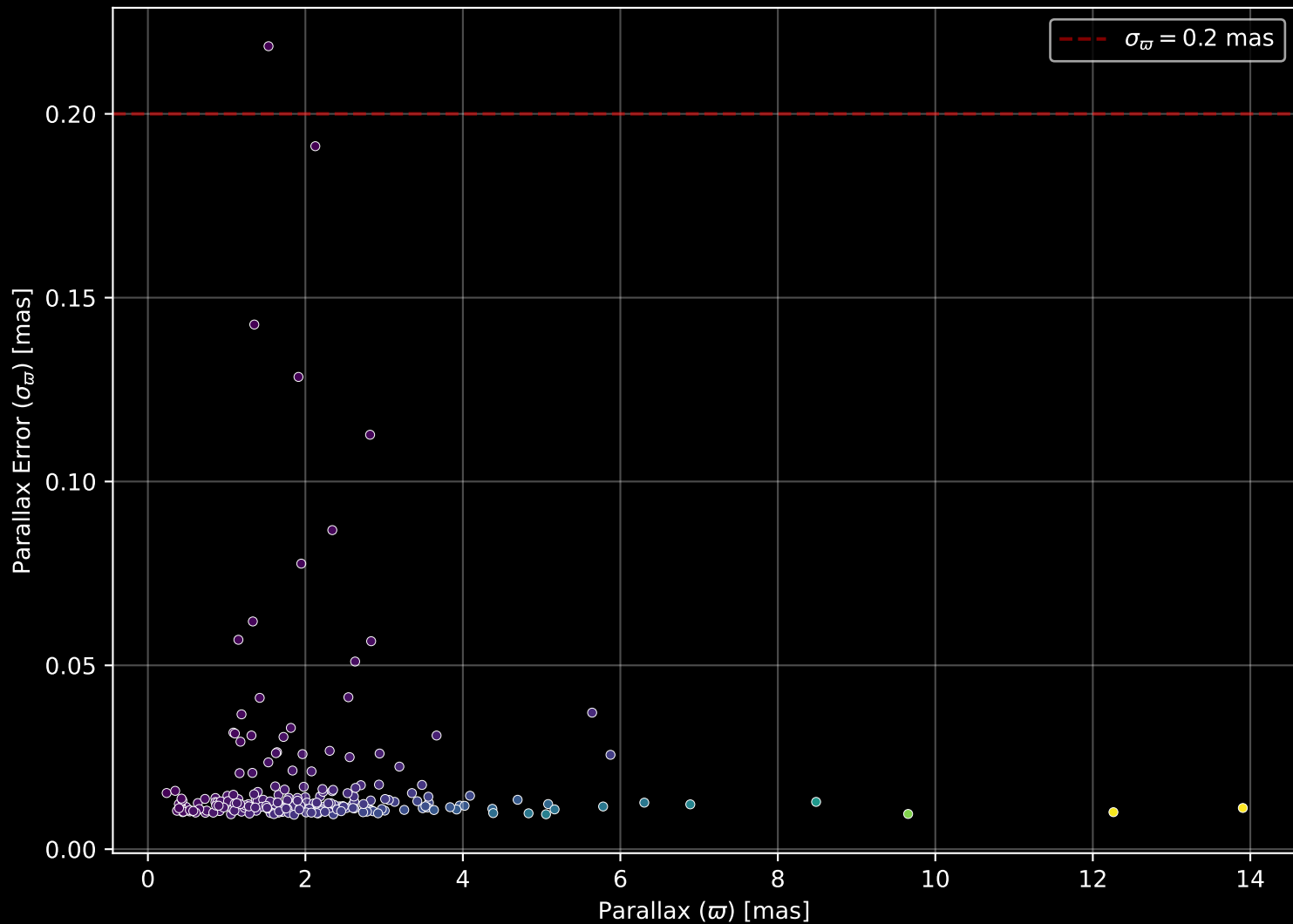
GALAH DR4 Field: [7133] Parallax Quality (n= 228)
