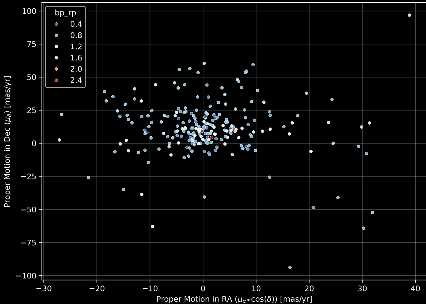
GALAH DR4 Field: [7133] Proper Motion Diagram (n= 228)
